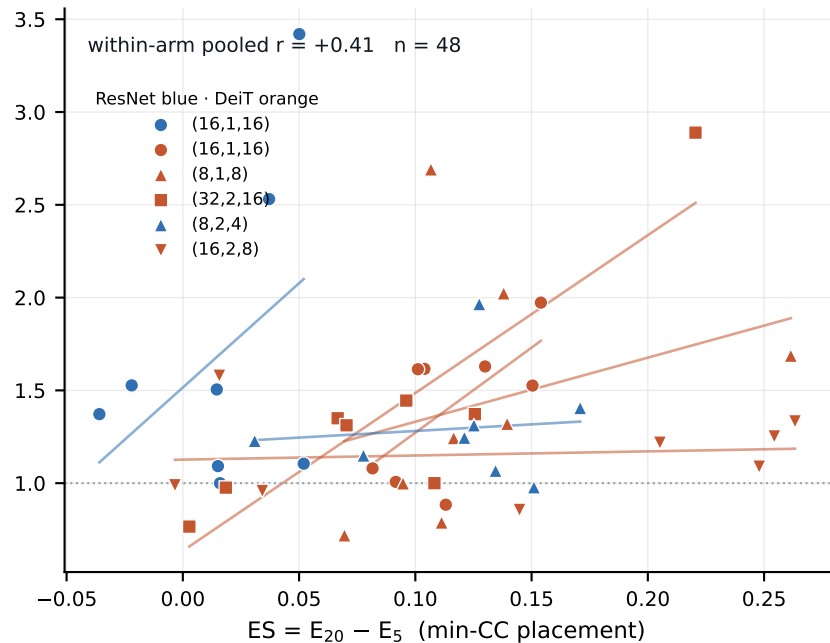
p99 runtime gain per placement
