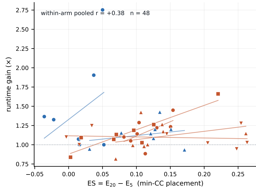
mean delay runtime gain per placement
