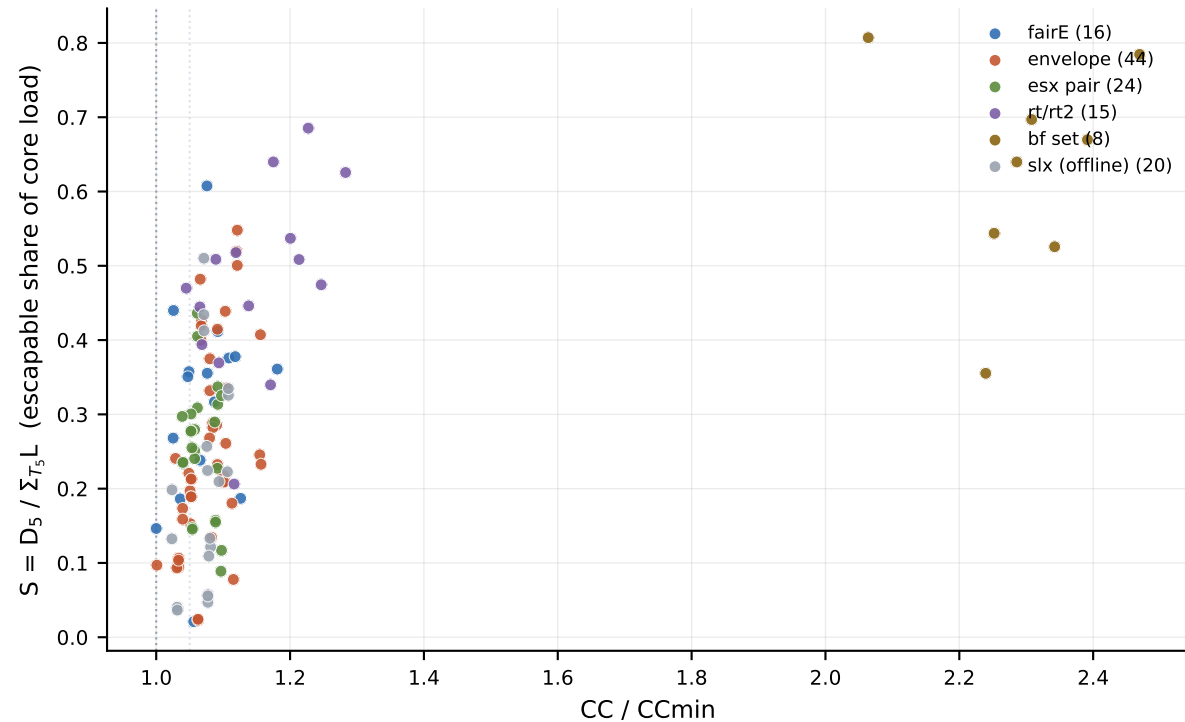
ResNet (8,2,4): escapable core share vs communication cost
