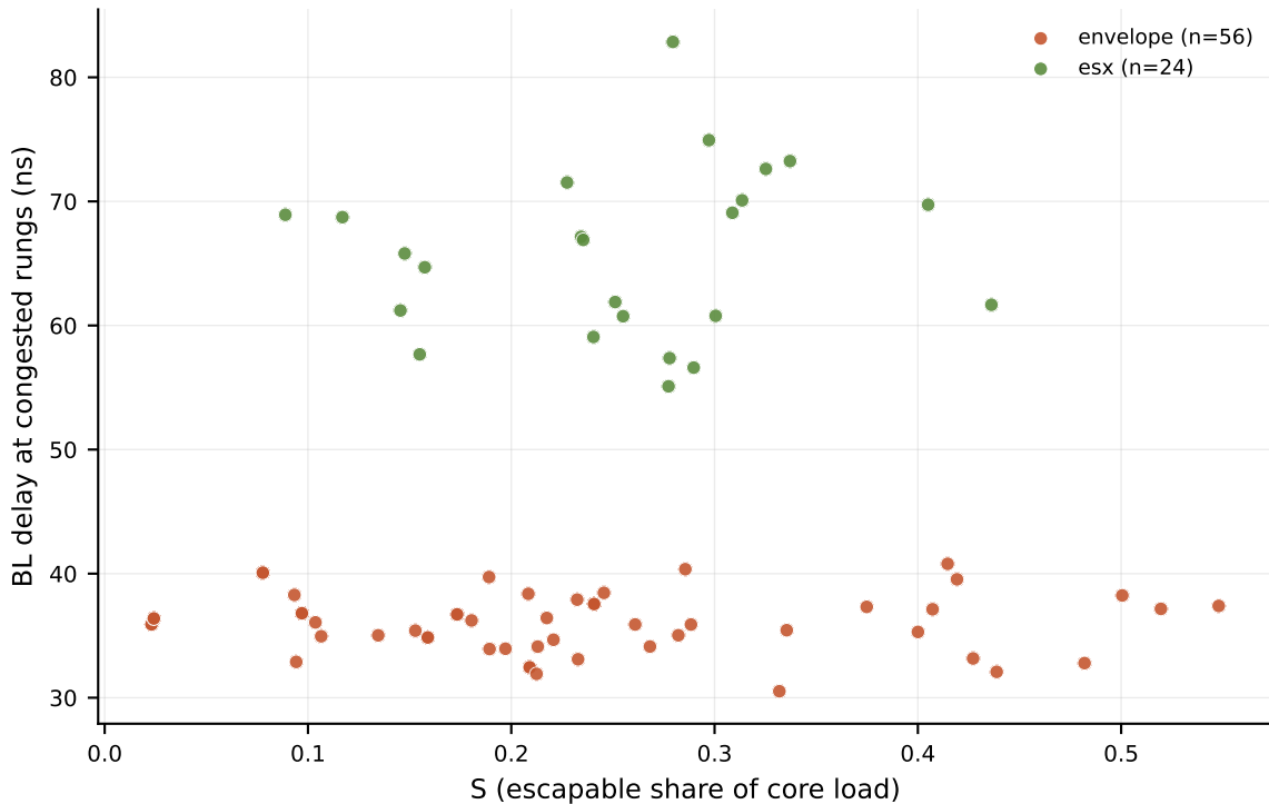
ResNet (8,2,4): measured delay vs S (CC within each campaign)
