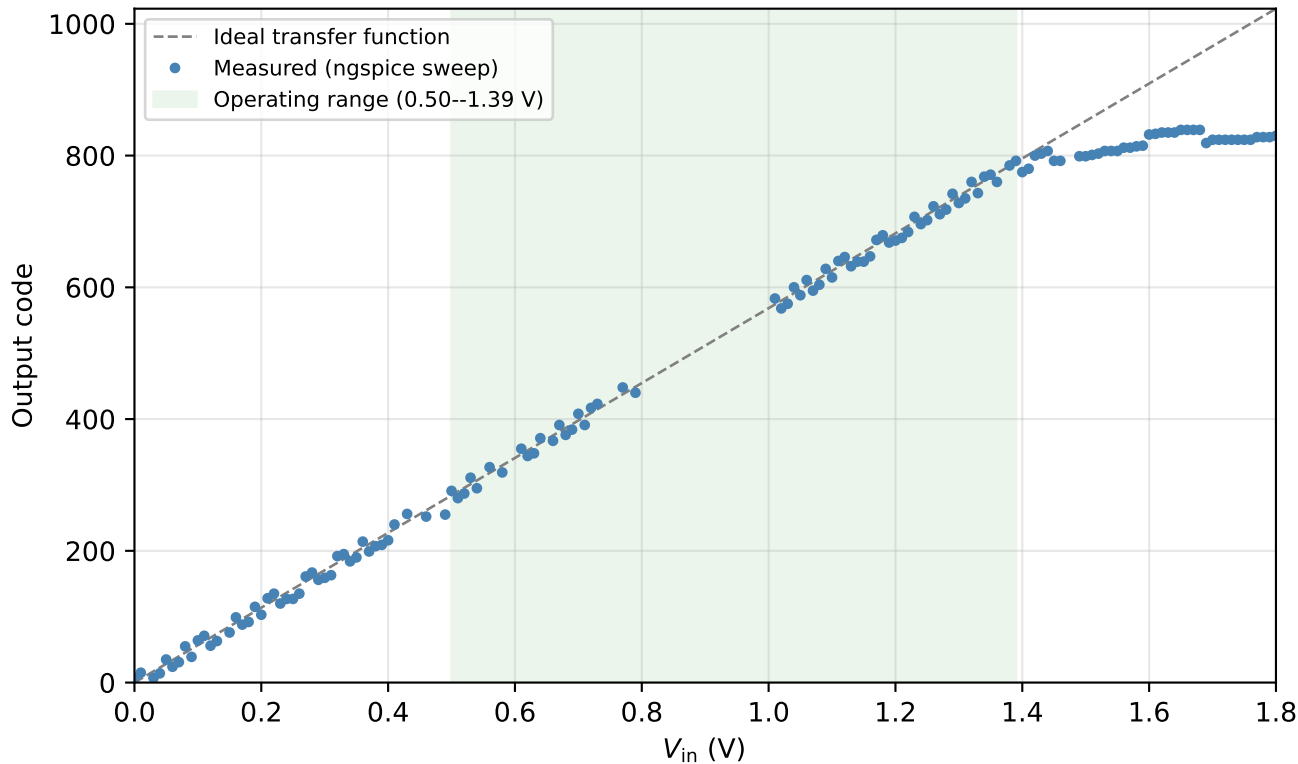
ADC Transfer Function, 10 mV DC Sweep
