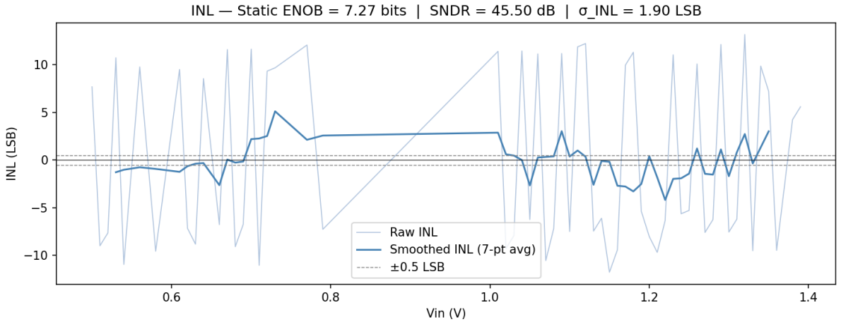
Figure 12: Raw and smoothed INL over the valid input range (0.50–1.39 V). The diagonal line visible in the raw curve near 0.79–1.01 V is an interpolation artefact caused by missing simulation points in that window, not a real feature of the transfer function. The +5 LSB peak in the smoothed curve near 0.75 V is caused by top-plate reset feedthrough from XTOP\_n , discussed further in Section 6.
