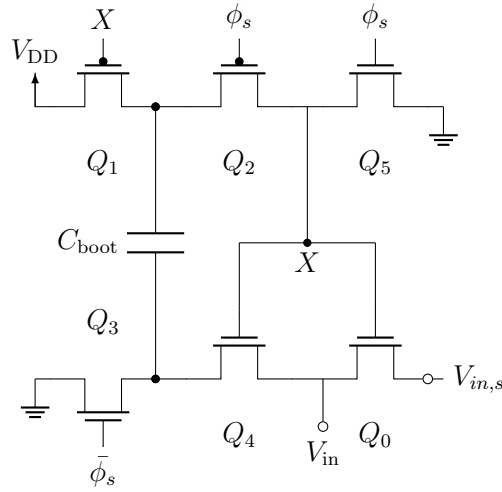
Figure 6: Bootstrapped sampling switch. Q_0 is the main sampling device; C_{\text{boot}} is precharged to V_{\text{DD}} during \bar{\phi}_s and bootstraps the gate of Q_0 to V_{\text{in}} + V_{\text{DD}} during \phi_s .
