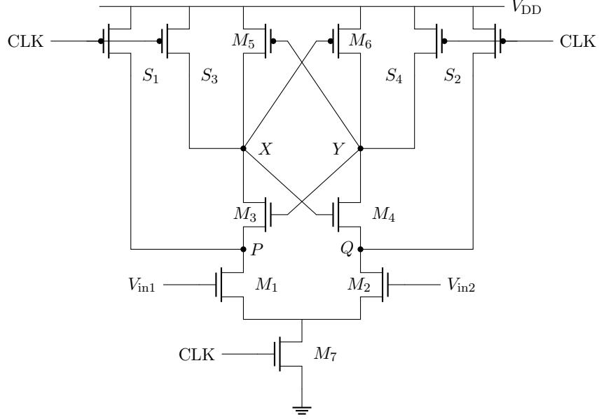
Figure 7: StrongARM latch comparator (Figure 1(b) from Razavi [3]). M1–M2 form the input differential pair, M3–M4 the cross-coupled NMOS latch, M5–M6 the cross-coupled PMOS latch, M7 the tail switch, and S1–S4 the precharge switches. Nodes P and Q are the intermediate amplification nodes; X and Y are the differential outputs.
