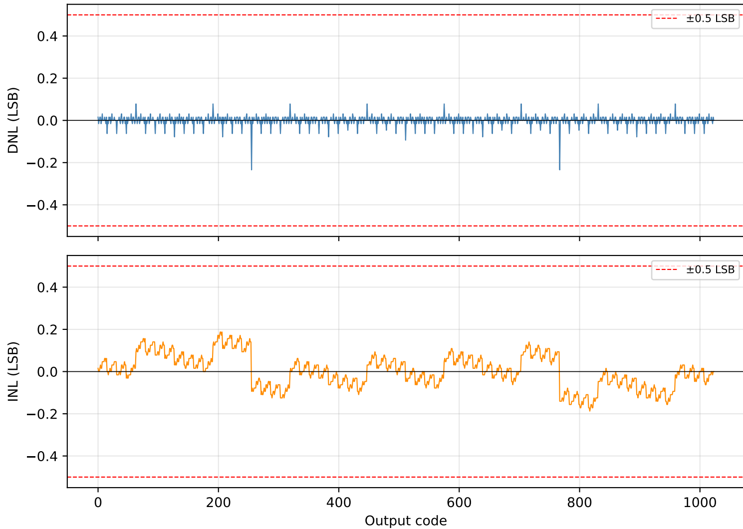
DNL and INL — single trial at C_{unit} = 25 fF, 2% mismatch
