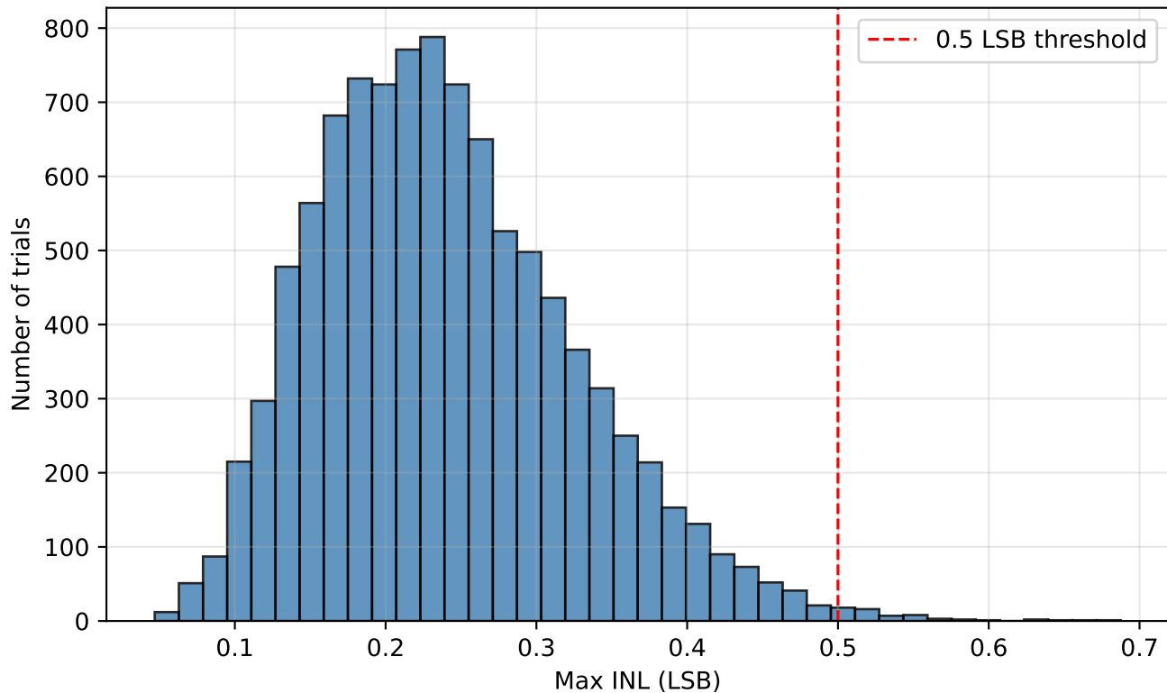
Max INL Distribution at C_{unit} = 25 fF — Yield: 99.4%
