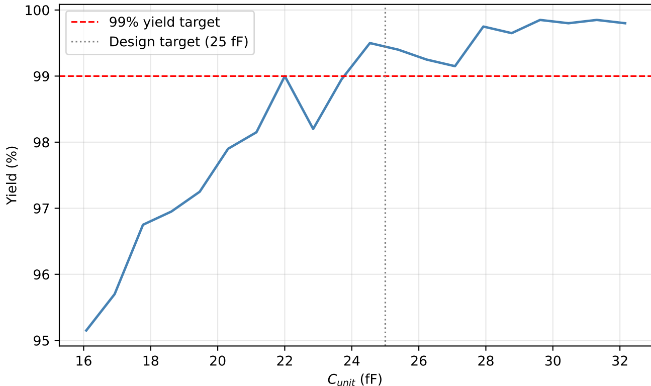
Yield vs Unit Capacitance (2% mismatch, 2000 trials)
