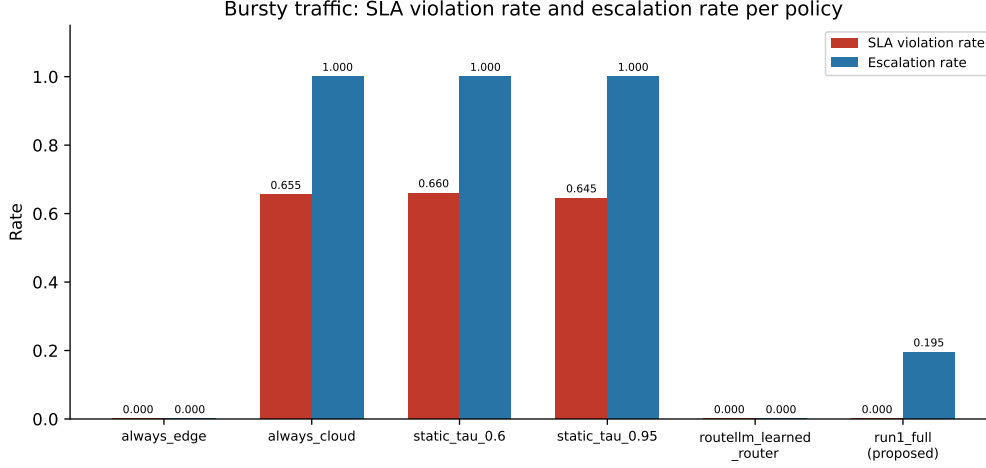
Figure 3: SLA violation rate and escalation rate per policy under bursty traffic (Table 7). Every static or always-cloud baseline that preserves accuracy pays for it with SLA violations in the 64.5–66.0% range; run1_full holds zero at roughly 19% of the escalation rate.
