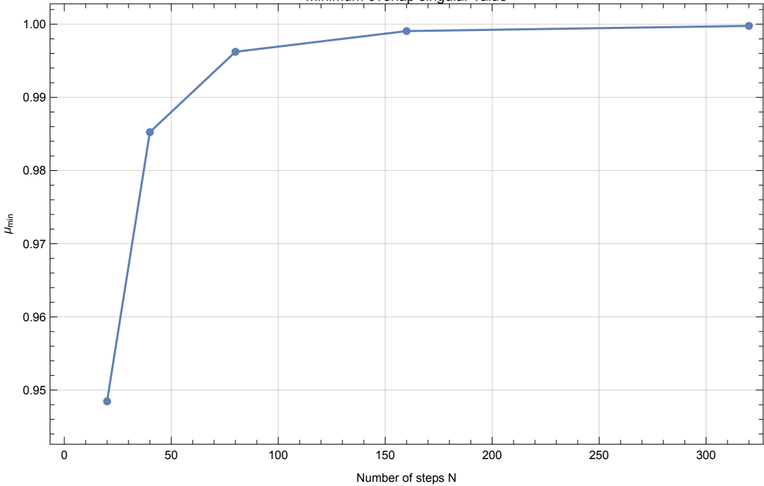
Minimum overlap singular value
