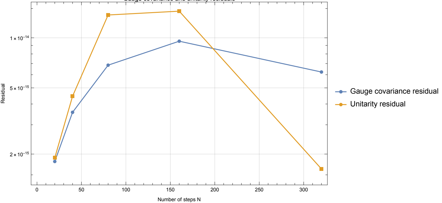
Gauge covariance and unitarity residuals
