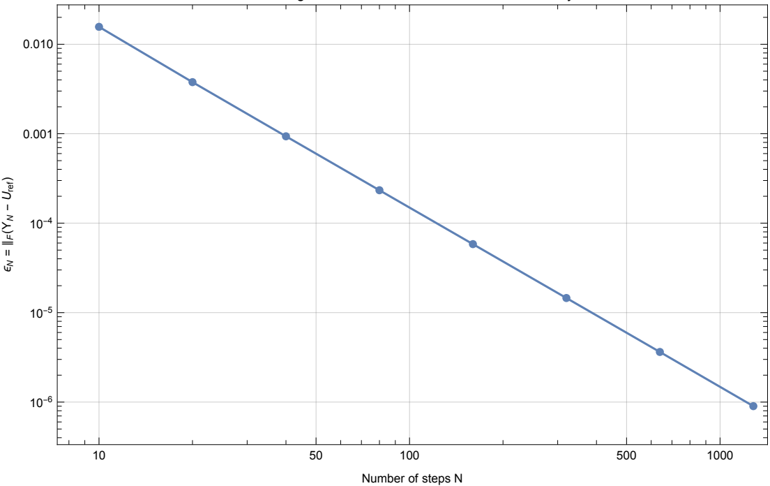
Convergence to continuum non-Abelian holonomy
