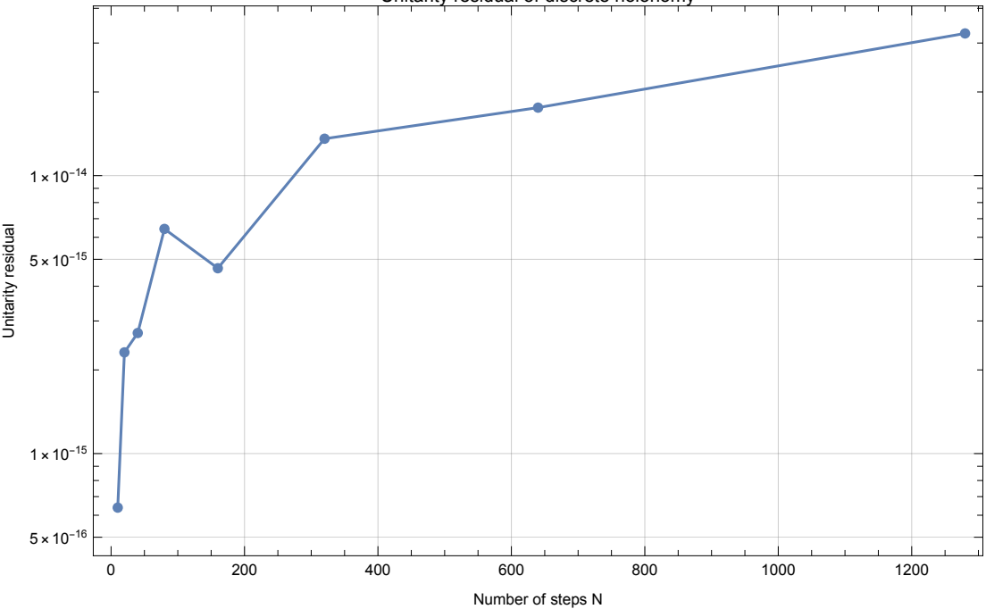
Unitarity residual of discrete holonomy
