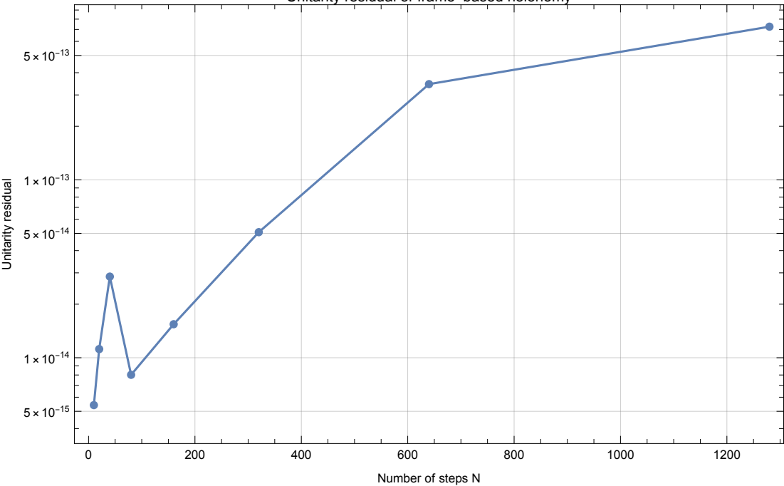
Unitarity residual of frame-based holonomy
