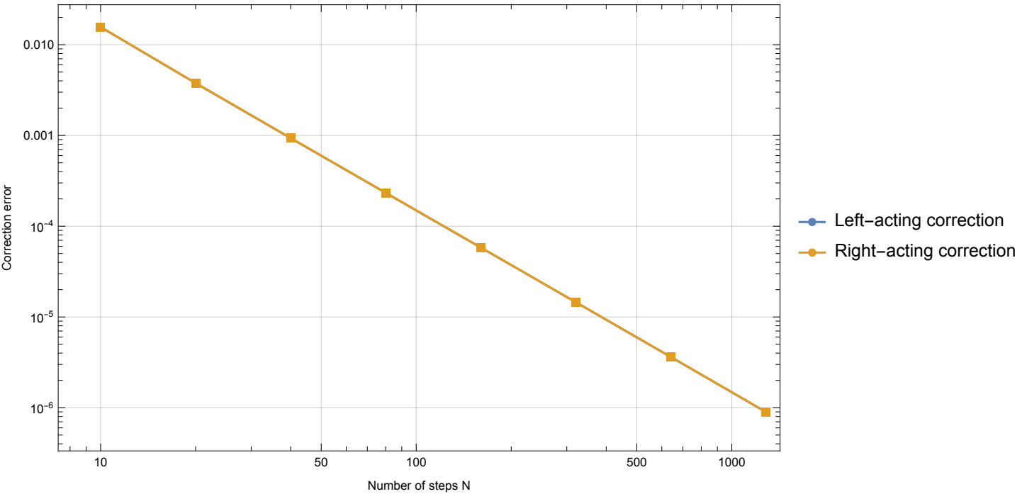
Feed-forward correction error
