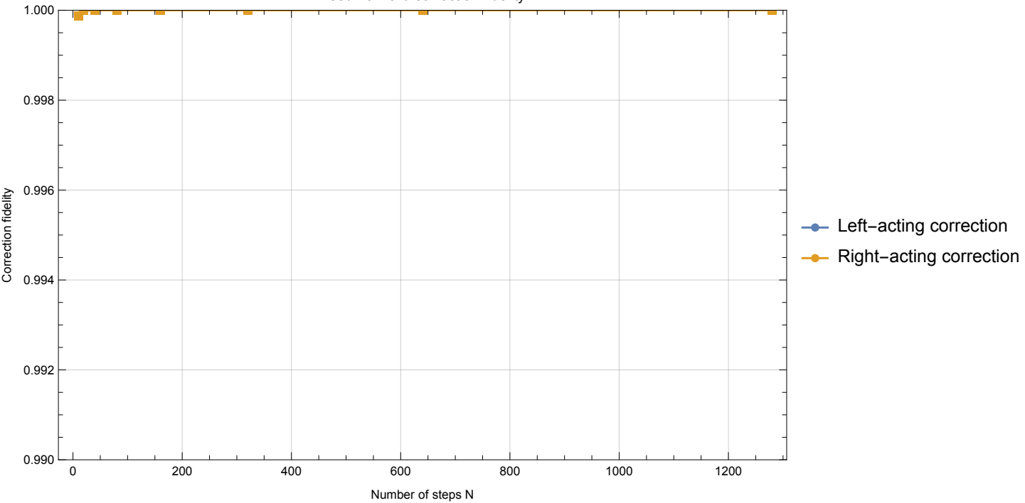
Feed-forward correction fidelity
