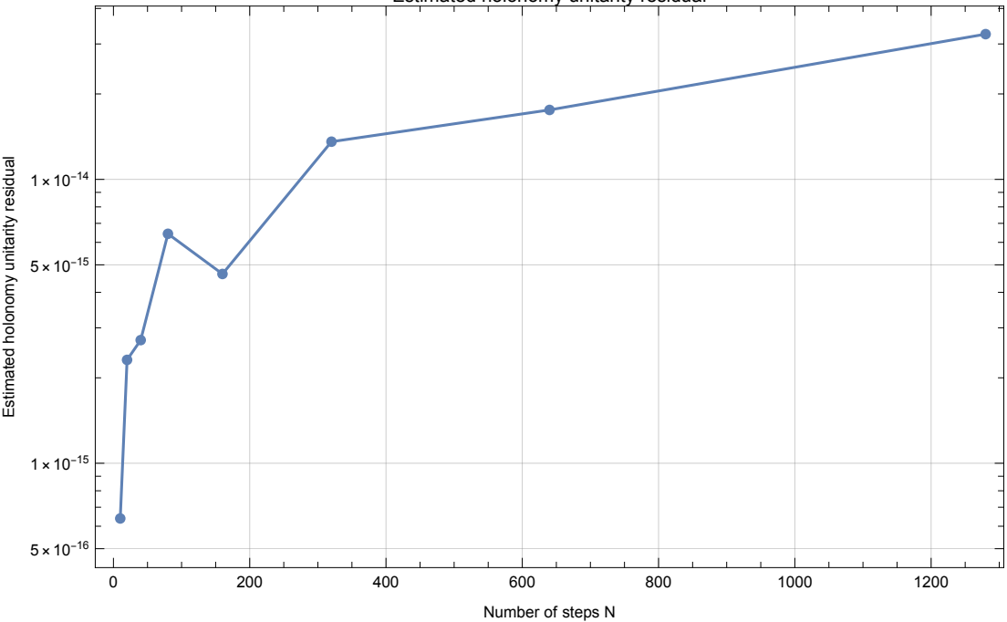
Estimated holonomy unitarity residual
