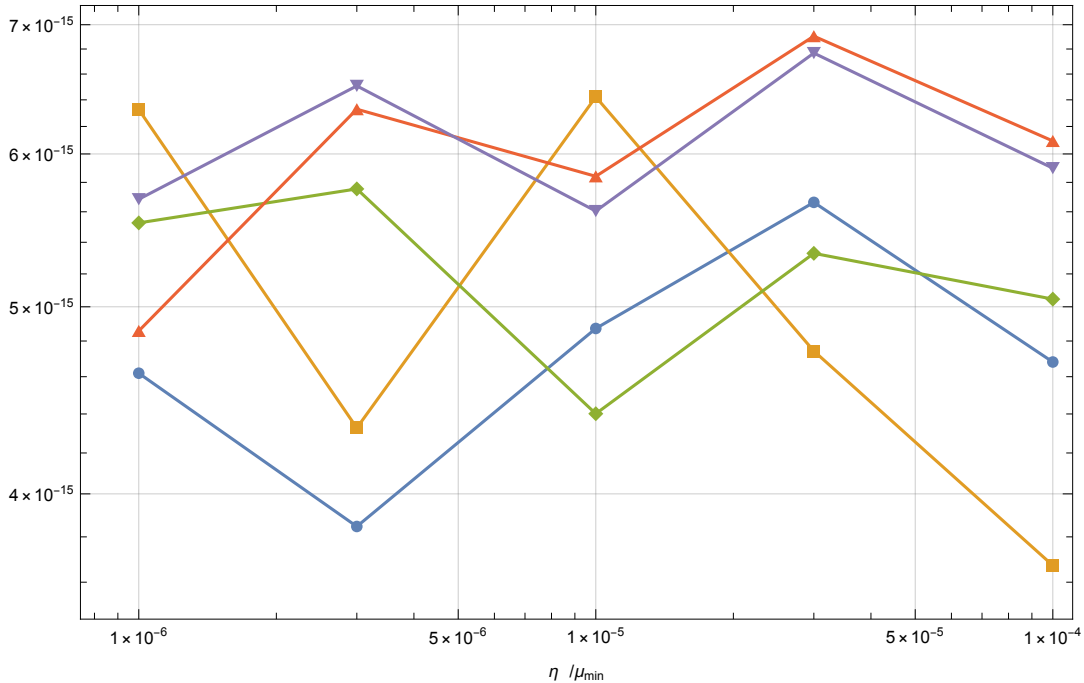
Unitarity residual under noisy overlaps
