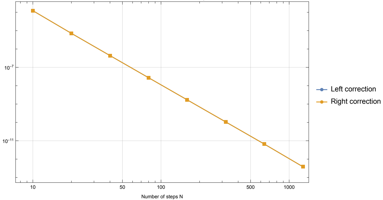
Feed-forward correction infidelity
