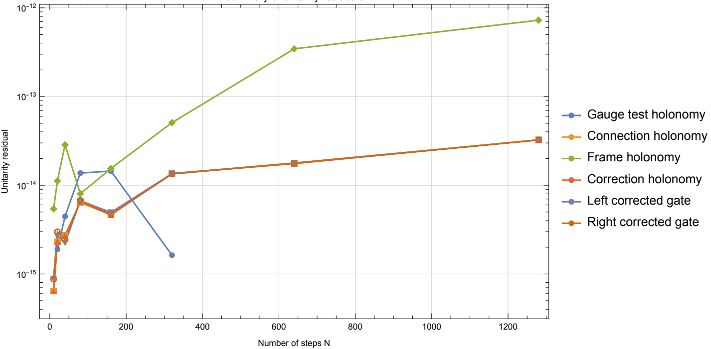
Summary of unitarity residuals
