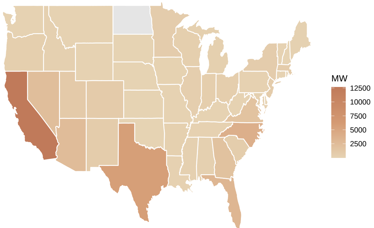
Mean Solar Capacity by State (MW)
