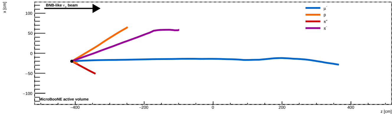
Event 0 primary-track projection in the beam plane
