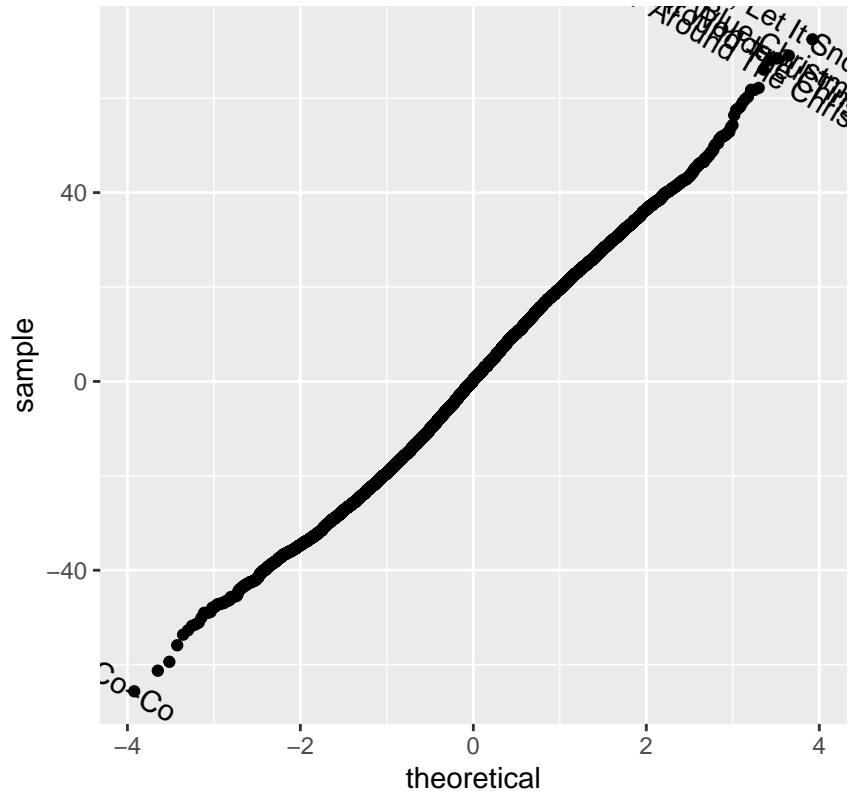
QQNorm Plot of Residuals
