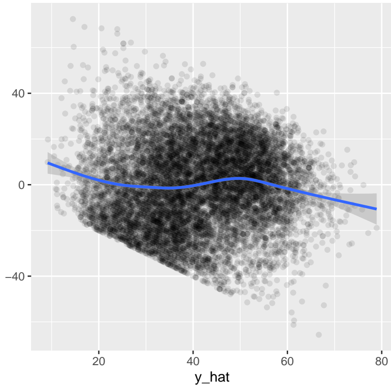
Residual Plot for GAM
