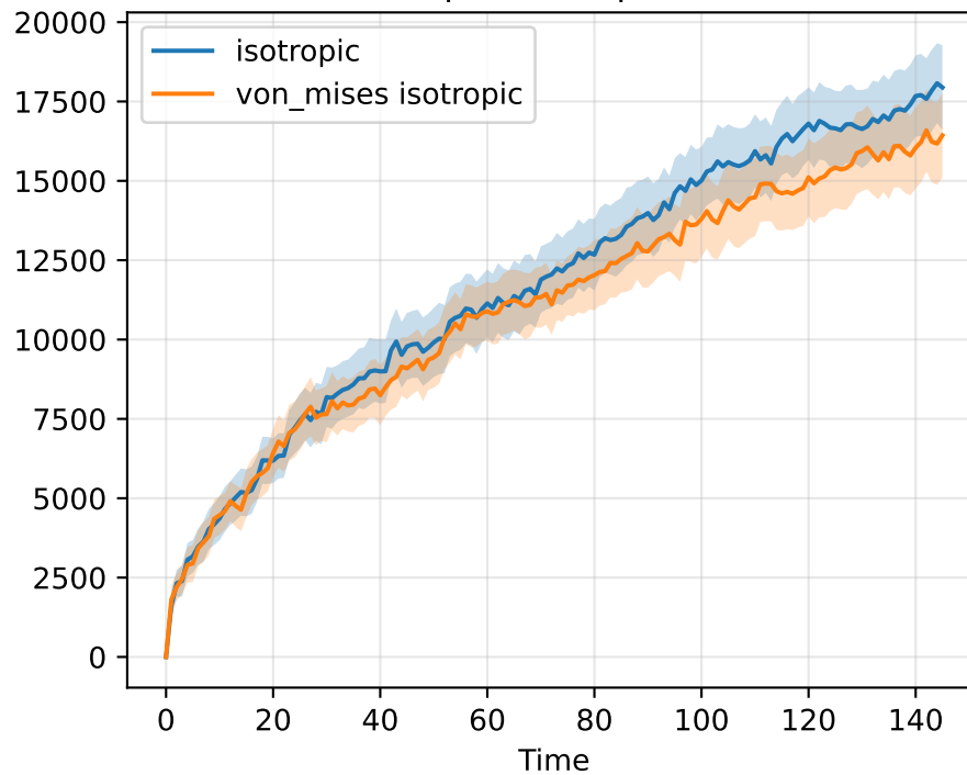
S0 (# clusters)
