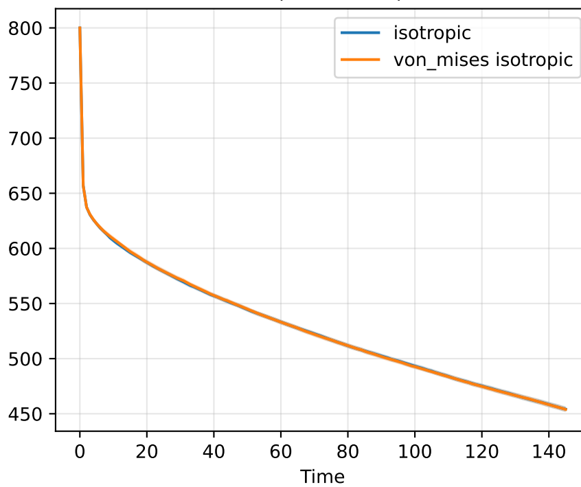
Largest cluster
