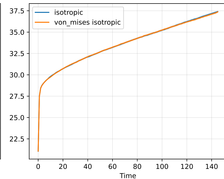
Mean NND
