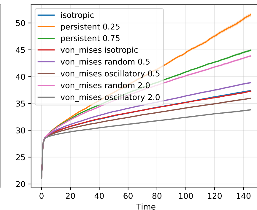
Mean NND
