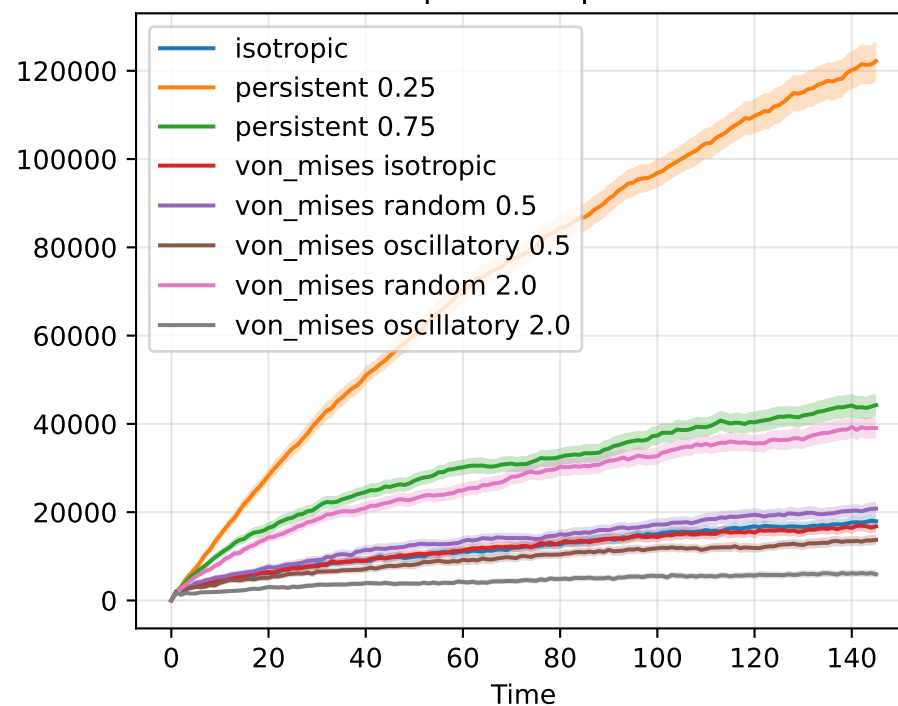
S0 (# clusters)
