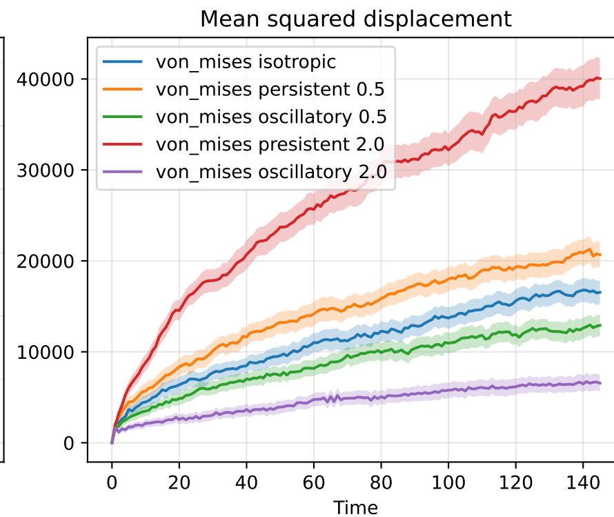
Angular model comparison: mean \pm 95% CI
