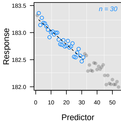
-- L pc Rank 1: y = 183.29 - 0.0252 \cdot x
