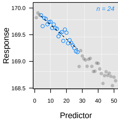
-- L pc Rank 1: y = 169.95 - 0.0269 \cdot x
