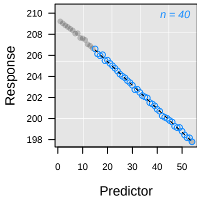
-- L_{pc} Rank 1: y = 209.86 - 0.2232 \cdot x
