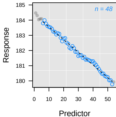
-- L_{pc} Rank 1: y = 184.39 - 0.0834 \cdot x
