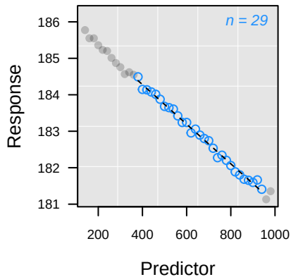
-- L_{pc} Rank 1: y = 186.45 - 0.0054 \cdot x
