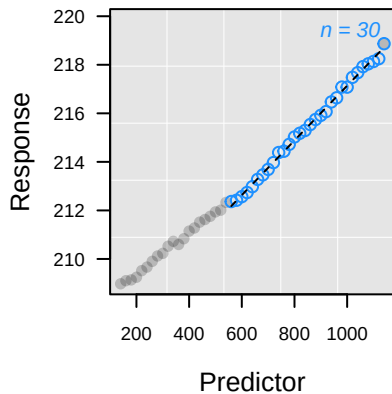
-- L_{pc} Rank 1: y = 205.87 + 0.0113 \cdot x
