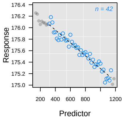
-- L_{pc} Rank 1: y = 176.41 - 0.0011 \cdot x
