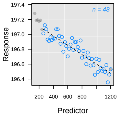
-- L_{pc} Rank 1: y = 197.23 - 0.0006 \cdot x
