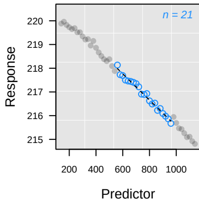
-- L pc Rank 1: y = 221.08 - 0.0055 \cdot x
