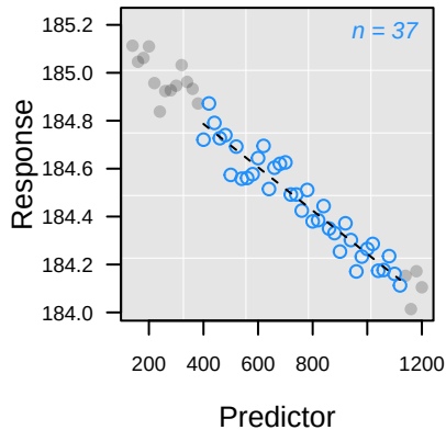
-- L_{pc} Rank 1: y = 185.15 - 0.0009 \cdot x
