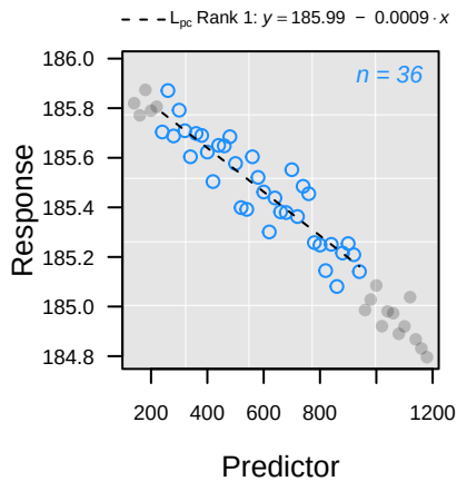
Sample quantiles
