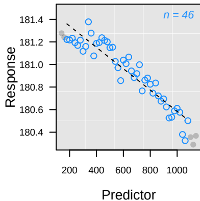
-- L_{pc} Rank 1: y = 181.53 - 0.0009 \cdot x
