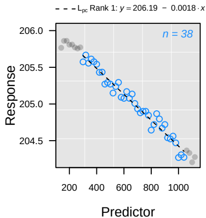
Sample quantiles
