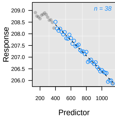
-- L_{pc} Rank 1: y = 209.72 - 0.0033 \cdot x
