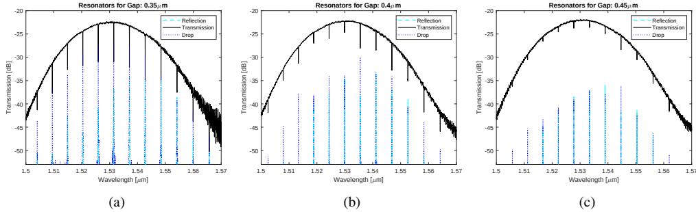
Fig. 11. Transmission for resonators with a) 0.35\ \mu\text{m} b) 0.40\ \mu\text{m} and c) 0.45\ \mu\text{m} gaps.
