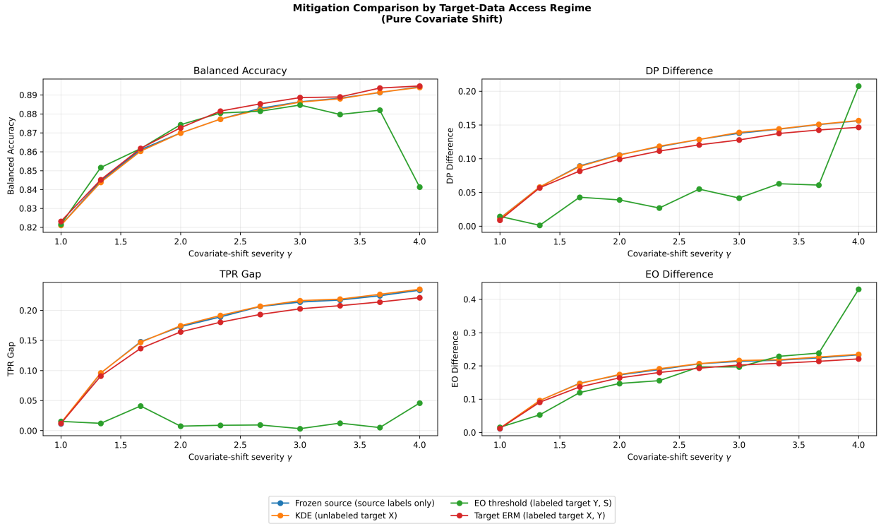
Figure 2: Mitigation comparison under pure covariate shift, organized by target-data access. KDE uses only unlabeled target covariates; equal-opportunity thresholding uses recorded target outcomes and group labels on a calibration set; target ERM uses labeled target training data. The methods are therefore access regimes rather than interchangeable fixes.
