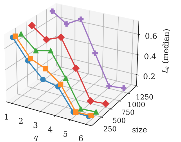
MBT18
