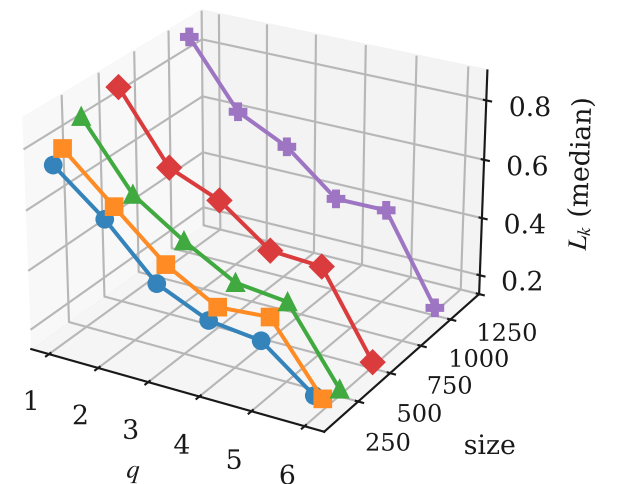
BMShj18-Hyper
