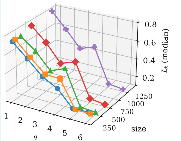
MBT18-Mean
