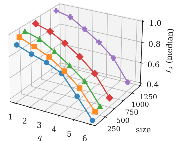
BMShj18-Fact
