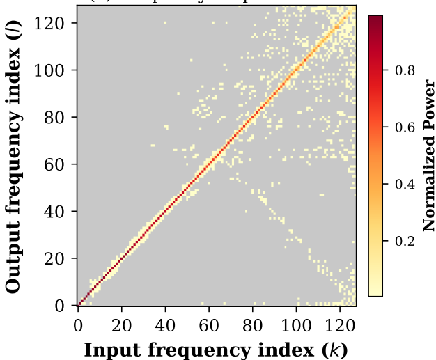
(a) Frequency-response matrix
