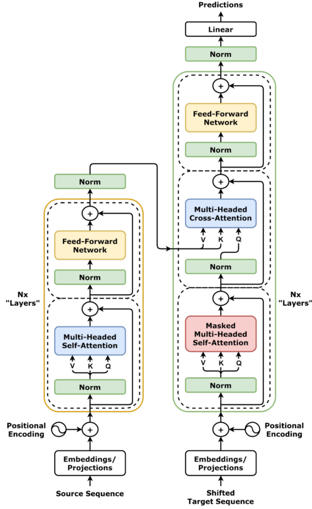
Figure 2.1: Transformer encoder-decoder architecture. The diagram shows the main building blocks used to transform input tokens into contextual representations and generated output tokens. [2]
