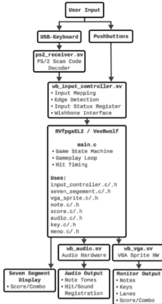
Figure 1: Block diagram showing all subsystems, user interface, and associated files.
