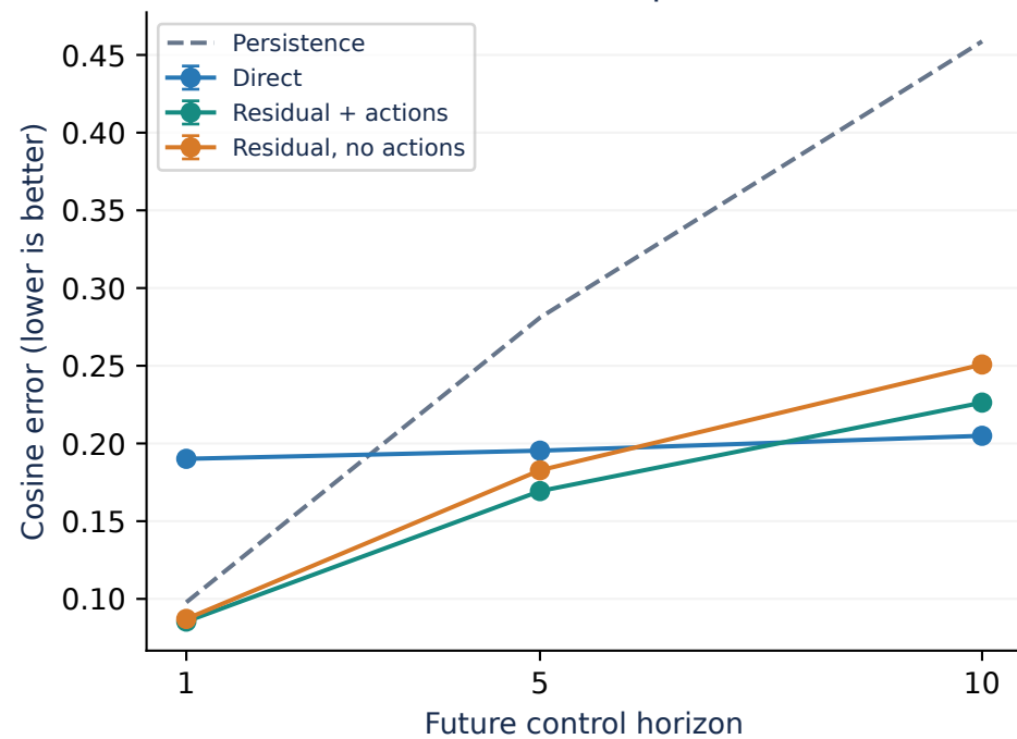
A Frozen-feature prediction
