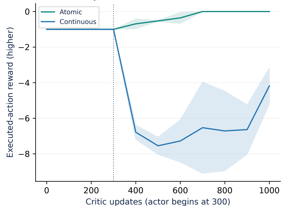
C Synthetic critic/actor stress test
