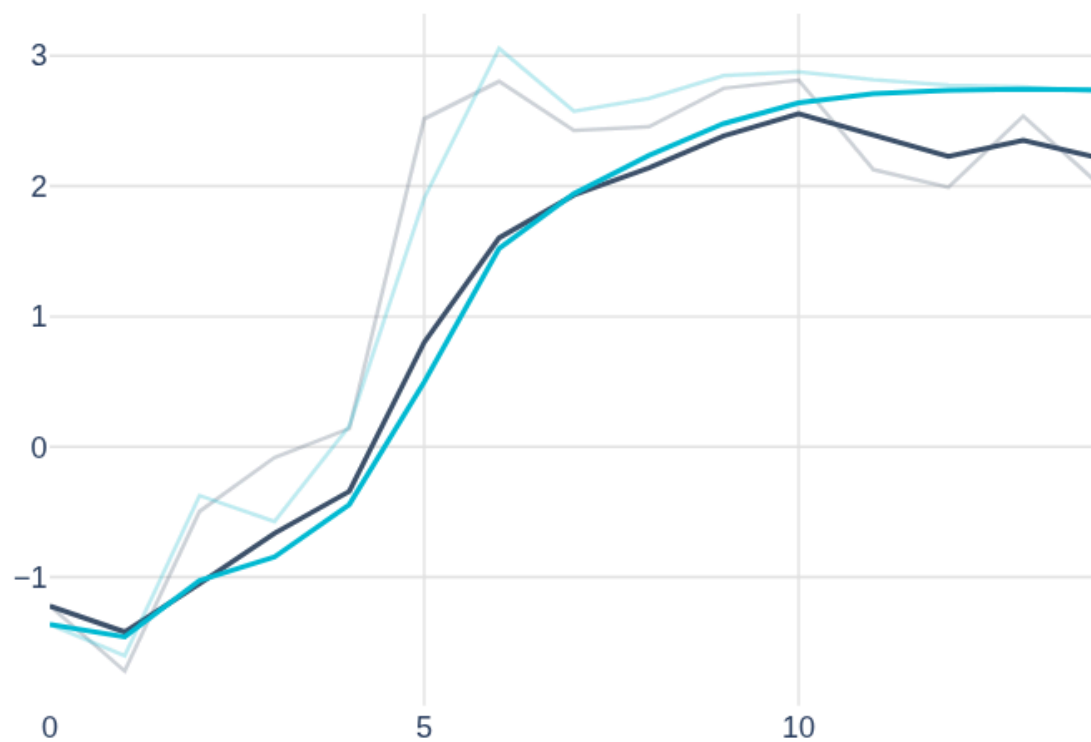
epoch_logit_mean
