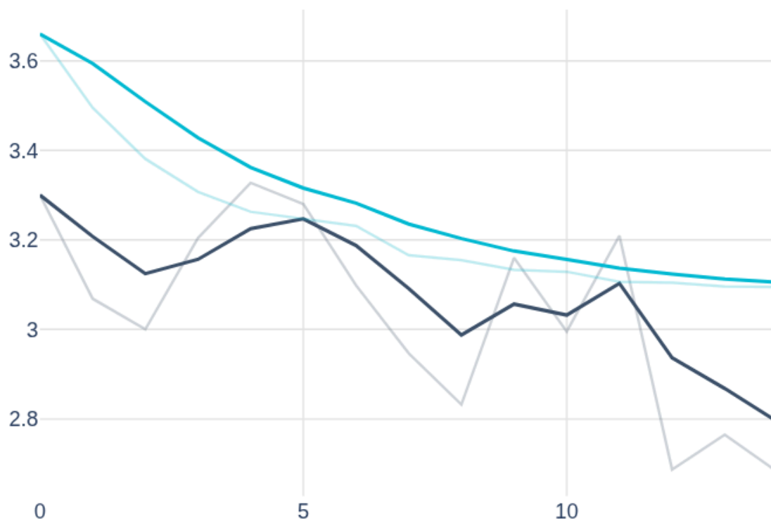
epoch_loss
