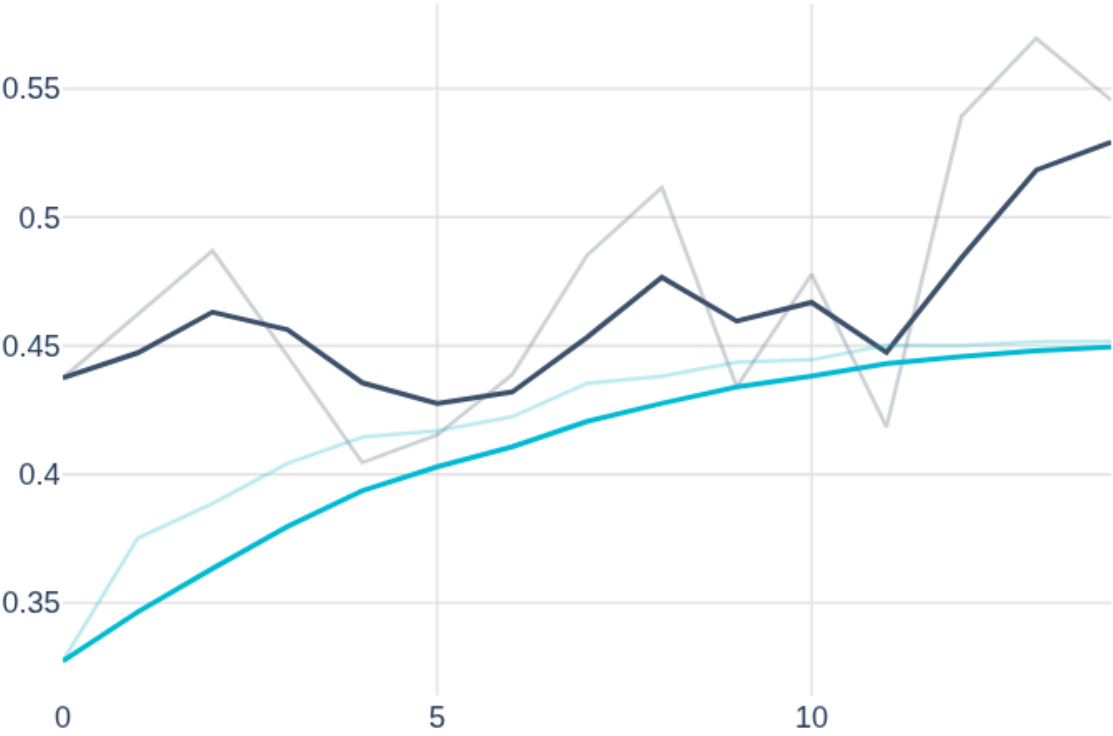
epoch_ndcg_20
