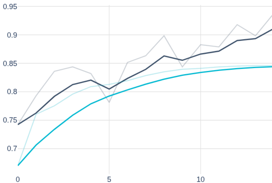
epoch_recall_20
