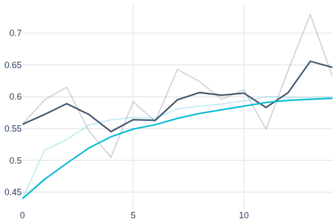
epoch_ndcg_head_20
