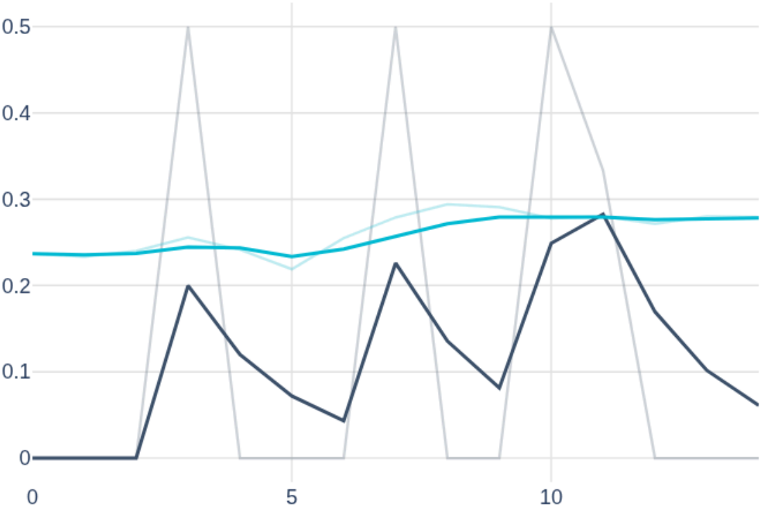
epoch_recall_tail_20
