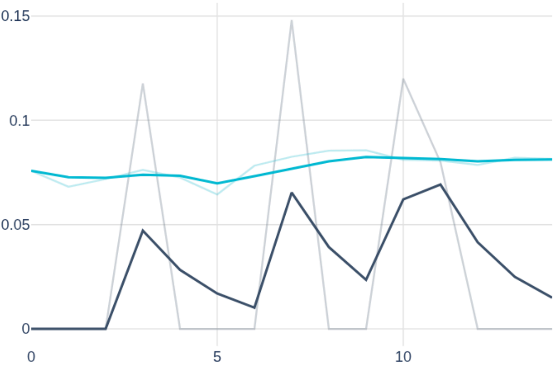
epoch_ndcg_tail_20
