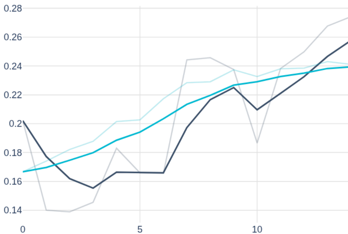
epoch_ndcg_torso_20
