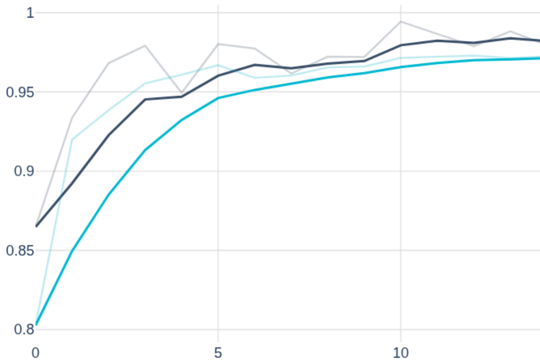
epoch_recall_head_20
