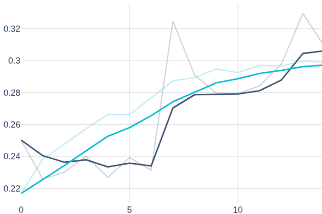
epoch_composite_ndcg_20
