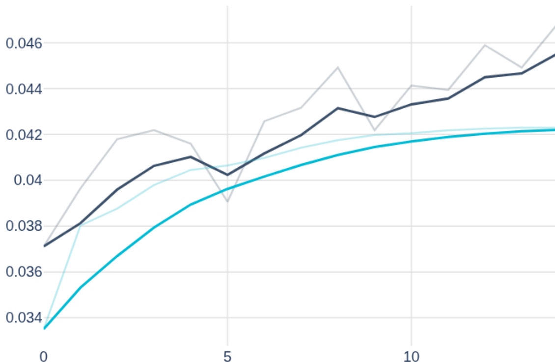
epoch_precision_20
