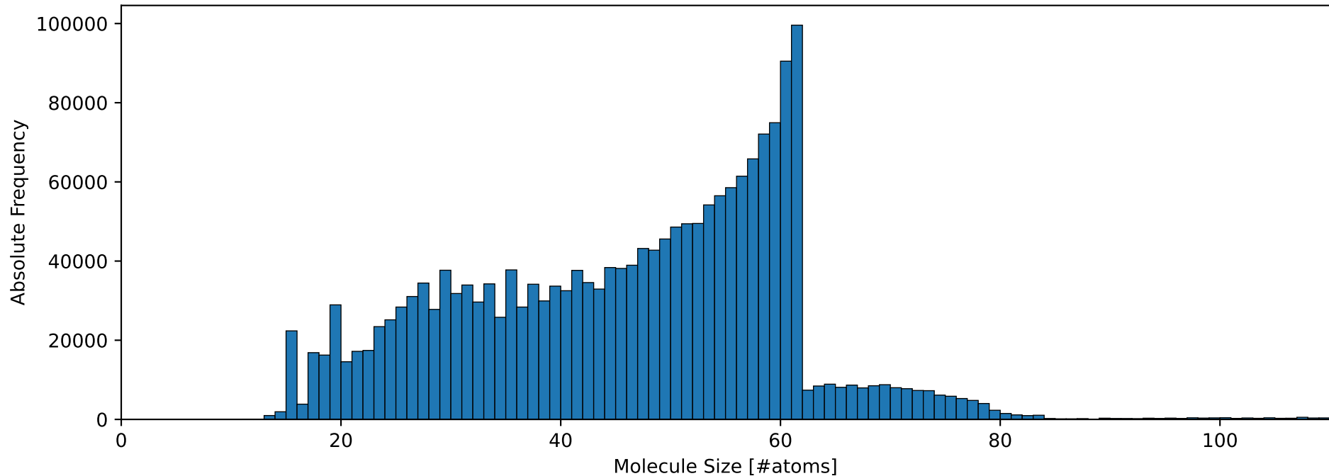
OMol25-SPICE Molecule Size Distribution
