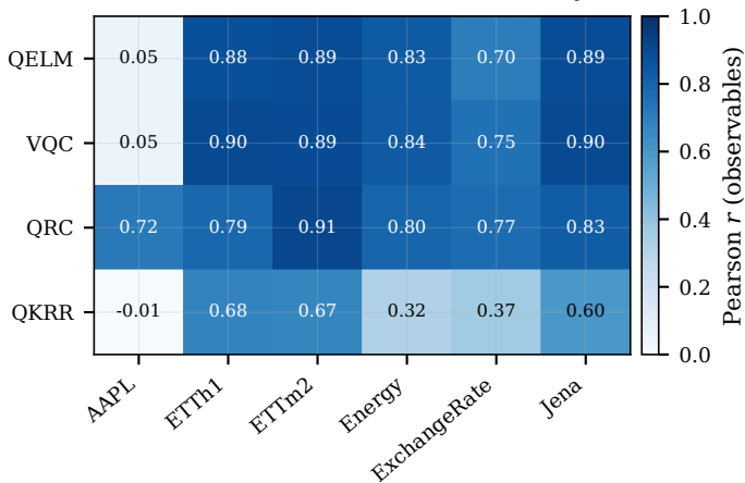
Student \rightarrow teacher observable fidelity
