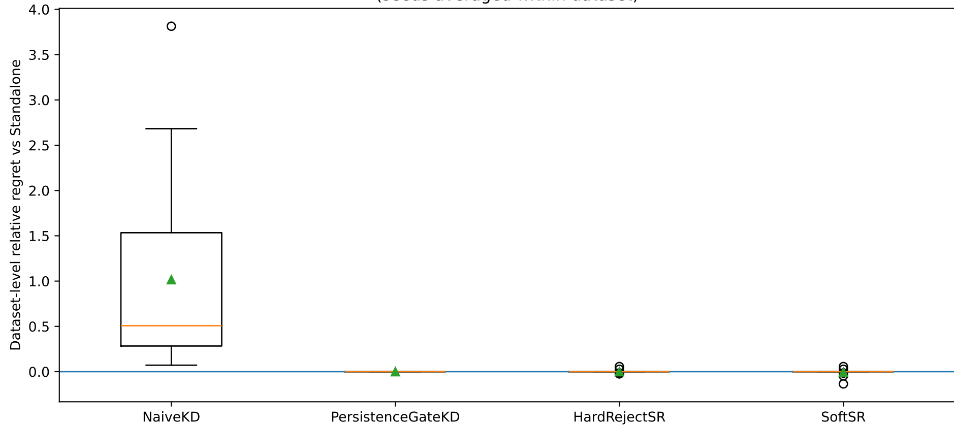
Quantum teachers: relative regret across dataset-teacher blocks (seeds averaged within dataset)
