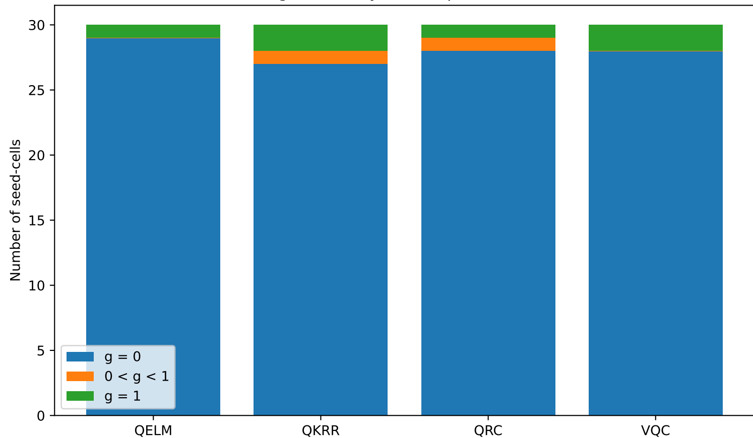
SoftSR gate activity across quantum teachers
